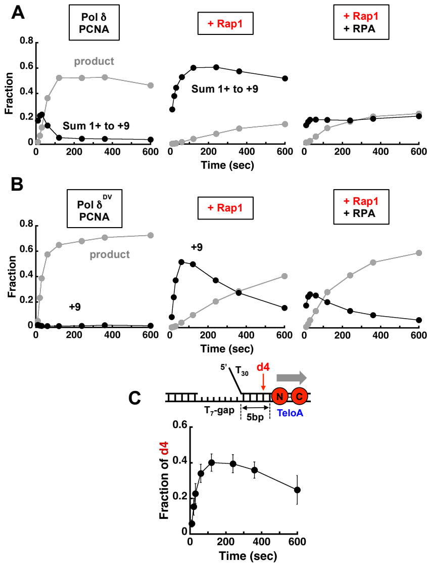
Figure S1. A single bound Rap1 is a barrier to the strand displacement activity of Pol \delta . A) Quantitation of the primer extension reactions in Figure 1B using Pol \delta . B) Quantitation of the primer extension reactions in Figure 1C using Pol \delta^{DV} . C) Reproducibility of the Rap1 block was tested in independent experiments (n=5) using the indicated substrate.
